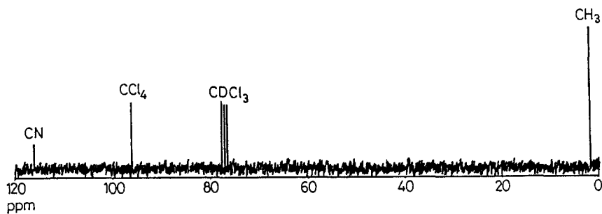
Fig. 2 ^{13}\text{C} NMR spectra performed in \text{CDCl}_3 with VARIAN XL300. From the right it may be seen the peak corresponding to \text{CH}_3 of acetonitrile, three peaks of \text{CDCl}_3 then the peaks respectively of \text{CCl}_4 and CN group
